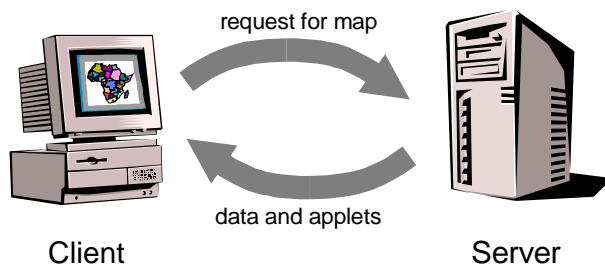
Figure III.6. Internet mapping – the client-side approach
